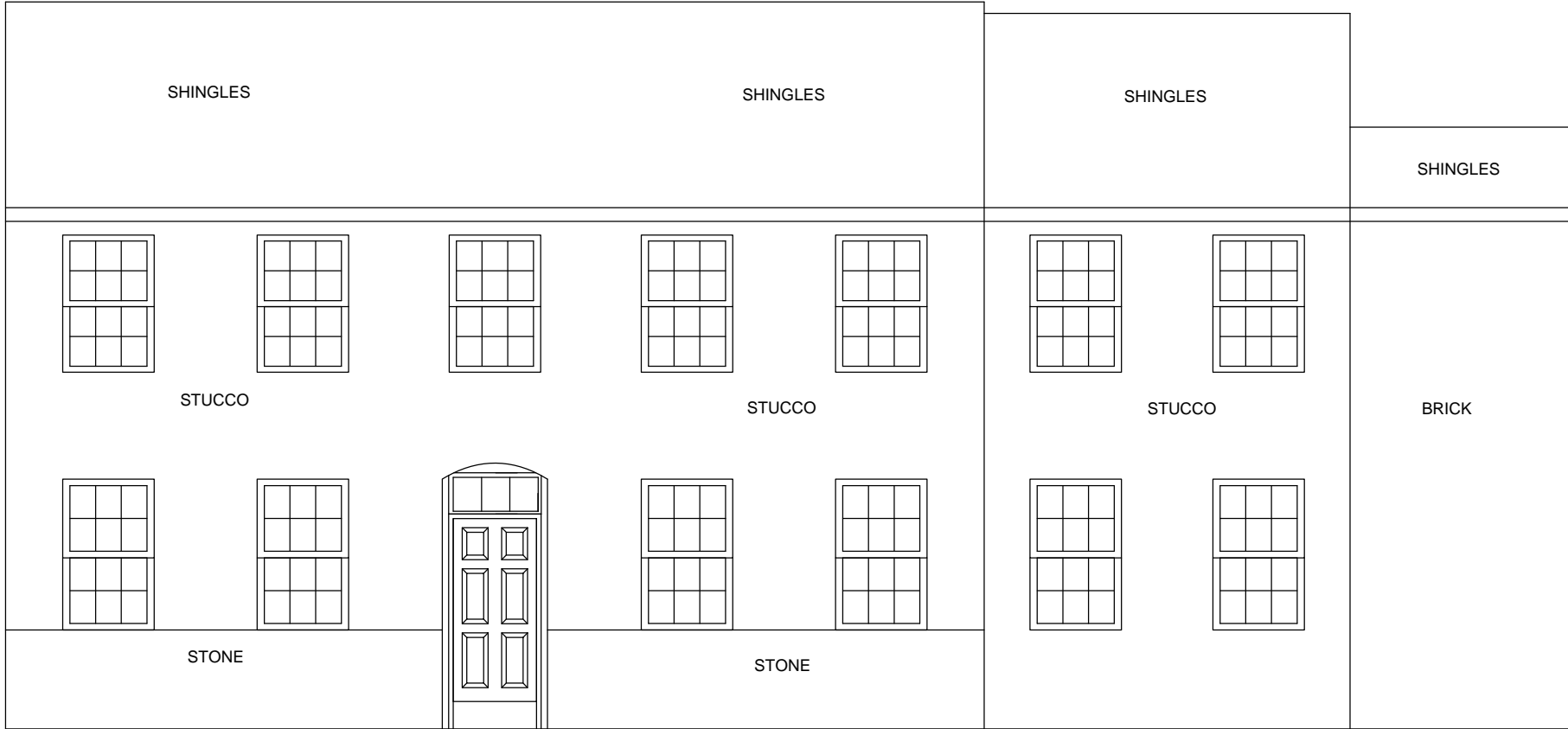
FRONT ELEVATION
