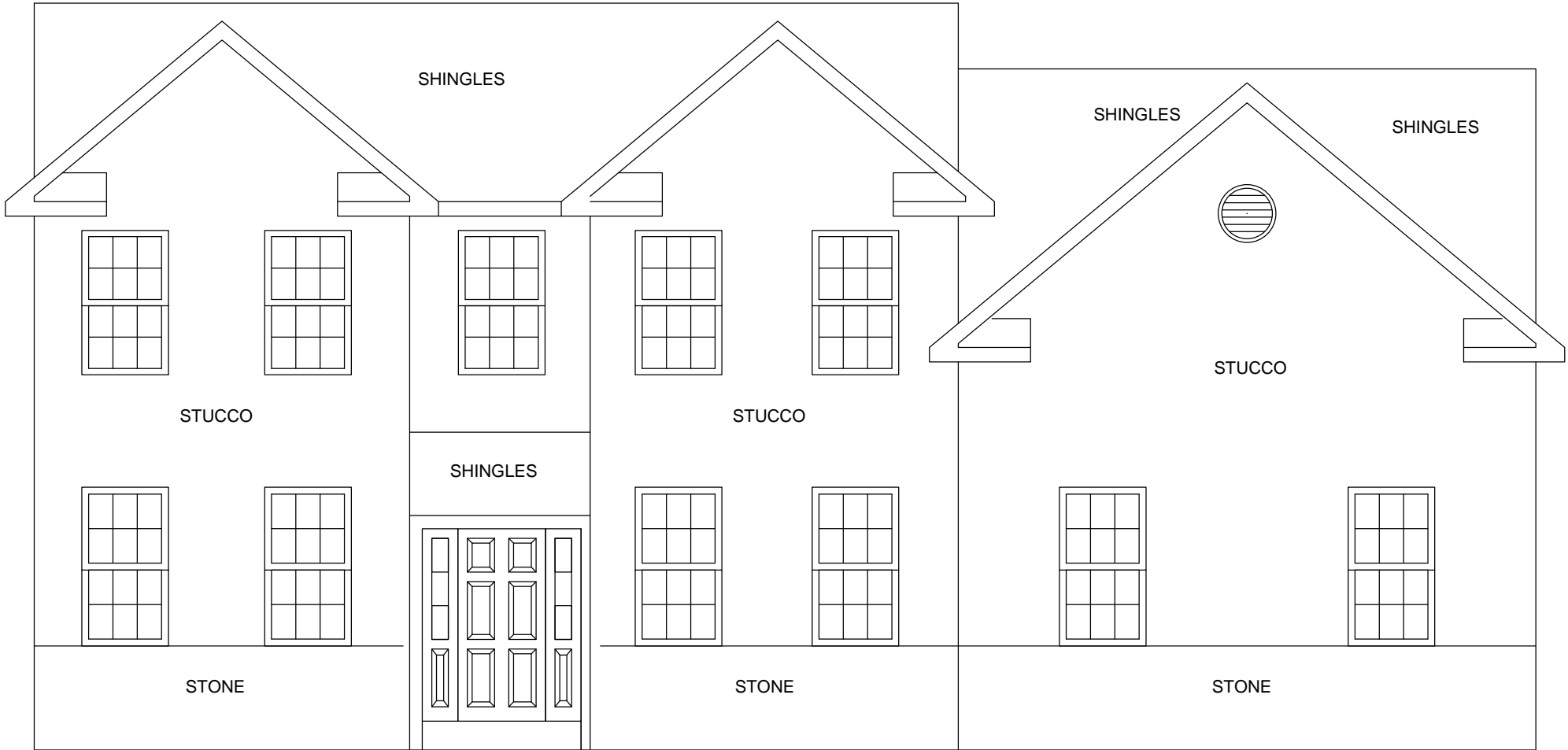
FRONT ELEVATION
